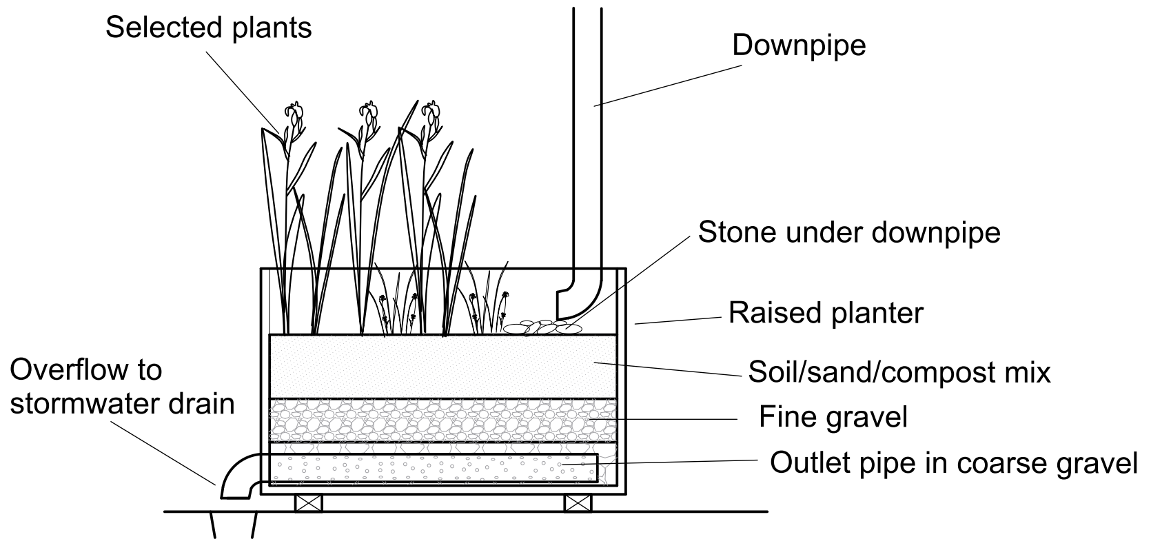
Raised Raingarden Planter
